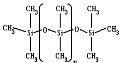
Polydimethylsiloxane
